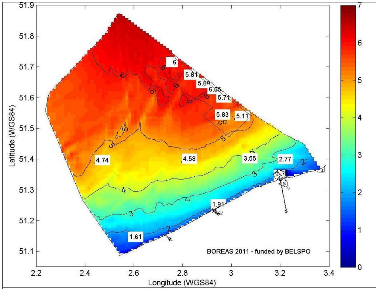
Figure 84: Average wave power (kW/m) for the year 2008 (final, with the 3 corrections).
